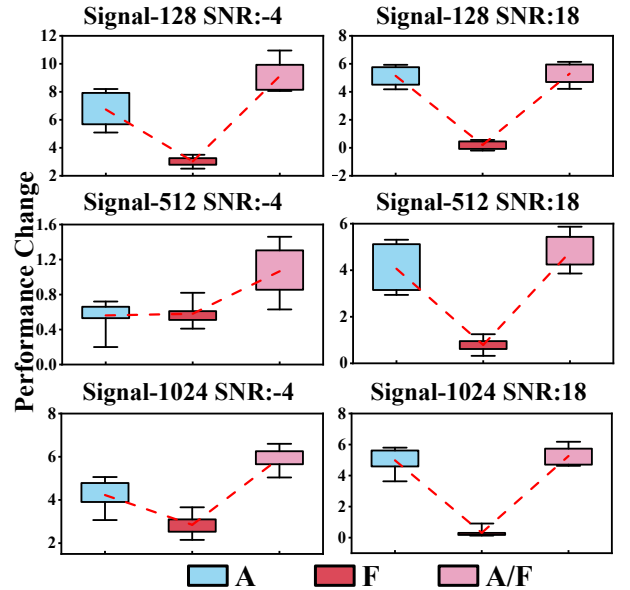
Fig. 3: Ablation study on 5-way-5-shot task for three datasets under two different SNR scenarios. ‘A’, ‘F’ represents the augmentation and noise filtering, respectively. The ‘A/F’ indicates the combination of augmentation and noise filtering. The dot line indicates the average performance change
