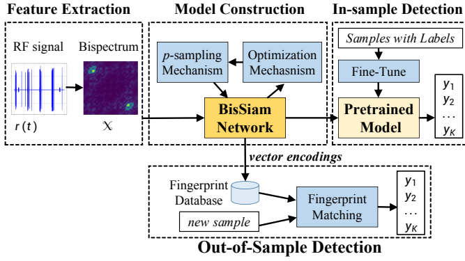
Fig. 3. The workflow of BISIAM
